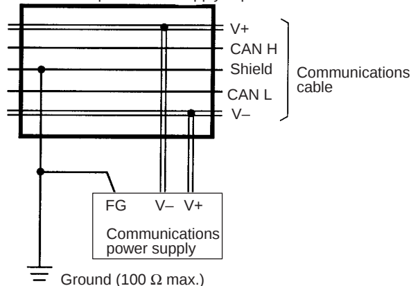
T-branch Tap or Power Supply Tap
