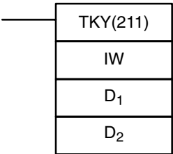
Ladder Symbols
